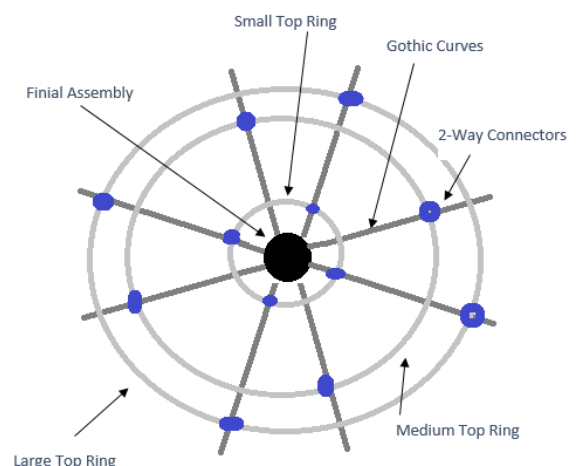
Figure 2: Attach the Top Rings
